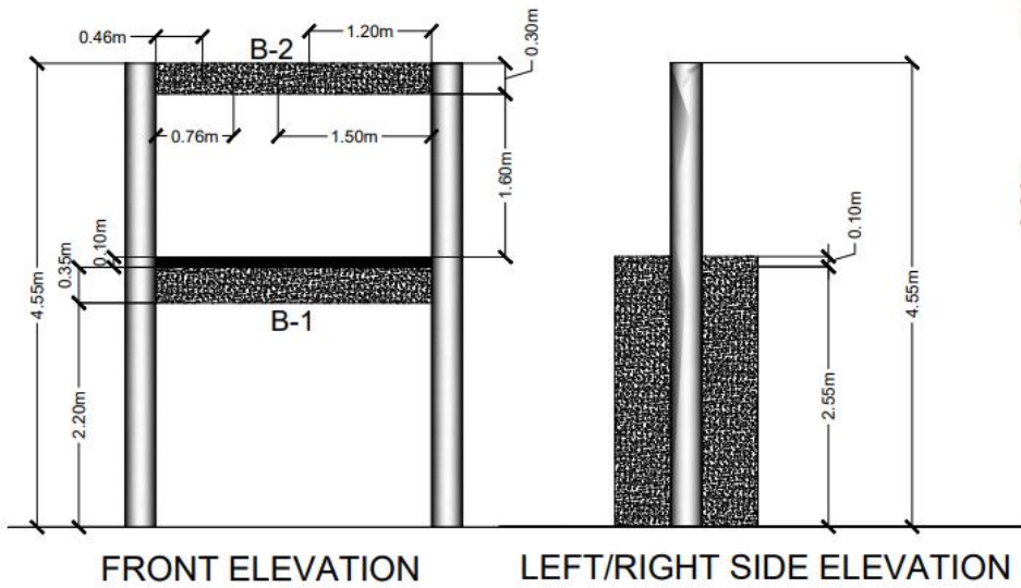
TRANSFORMER PLATFORM DETAIL
