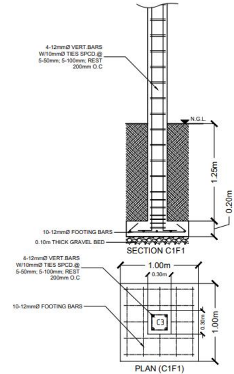
PLAN (C1F1)
