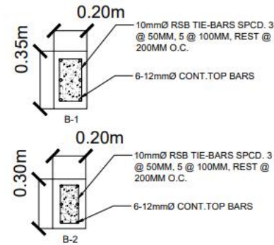
BEAM DETAILS
