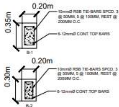
BEAM DETAILS SCALE 1:20 M
