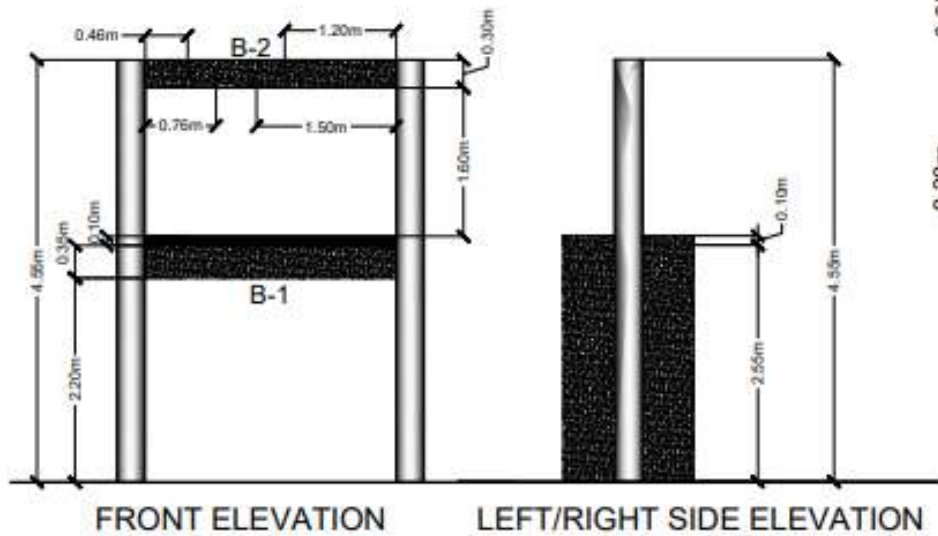
BEAM DETAILS SCALE 1:20 M
