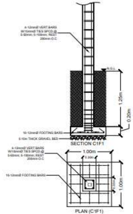
COLUMN FOOTING (C1F1) DETAIL SCALE 1:30 M
