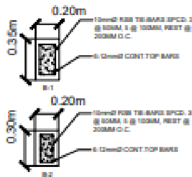
BEAM DETAILS
