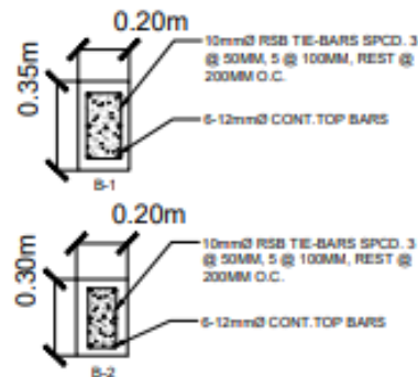
BEAM DETAILS
